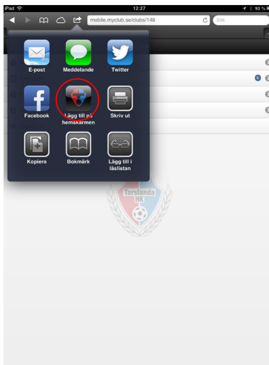
Figur 1: iOS
